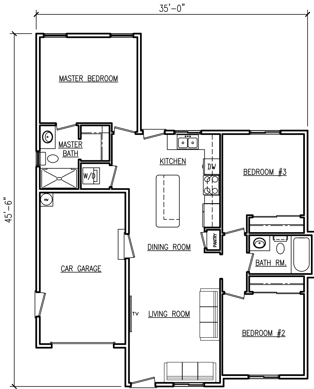
THE NEWBERG PLAN TOTAL LIVING = 1031 SQ.FT.
