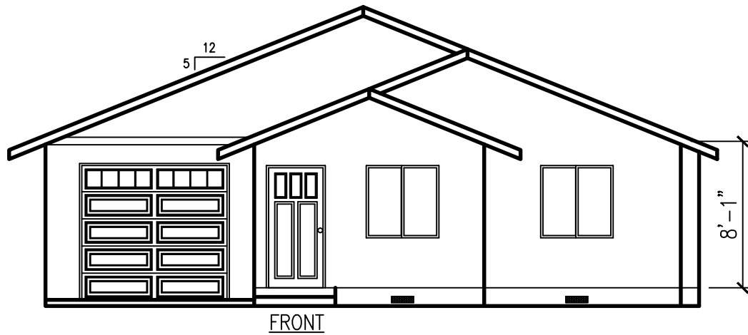
THE NEWBERG PLAN TOTAL LIVING = 1031 SQ.FT.
